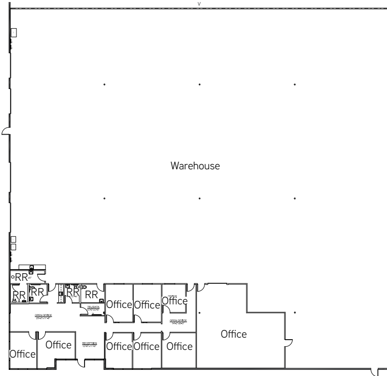
Floor Plan
